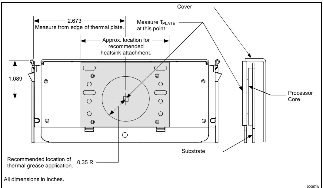
Figure 19. Processor Thermal Plate Temperature Measurement Location
