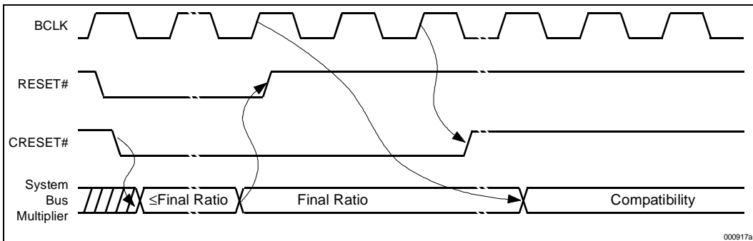
Figure 4. Timing Diagram of System Bus Multiplier Signals
