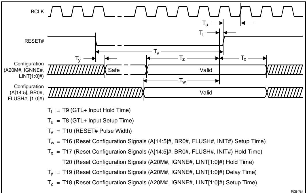
Figure 11. System Bus Reset and Configuration Timings
