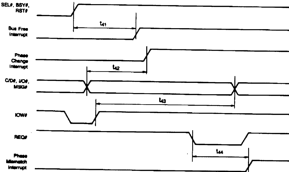
Fig 9. SCSI Bus free Detection and Phase Change Interrupts
