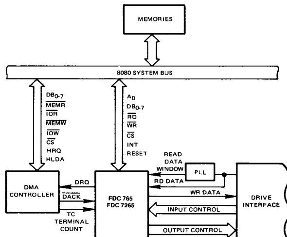
SYSTEM CONFIGURATION
