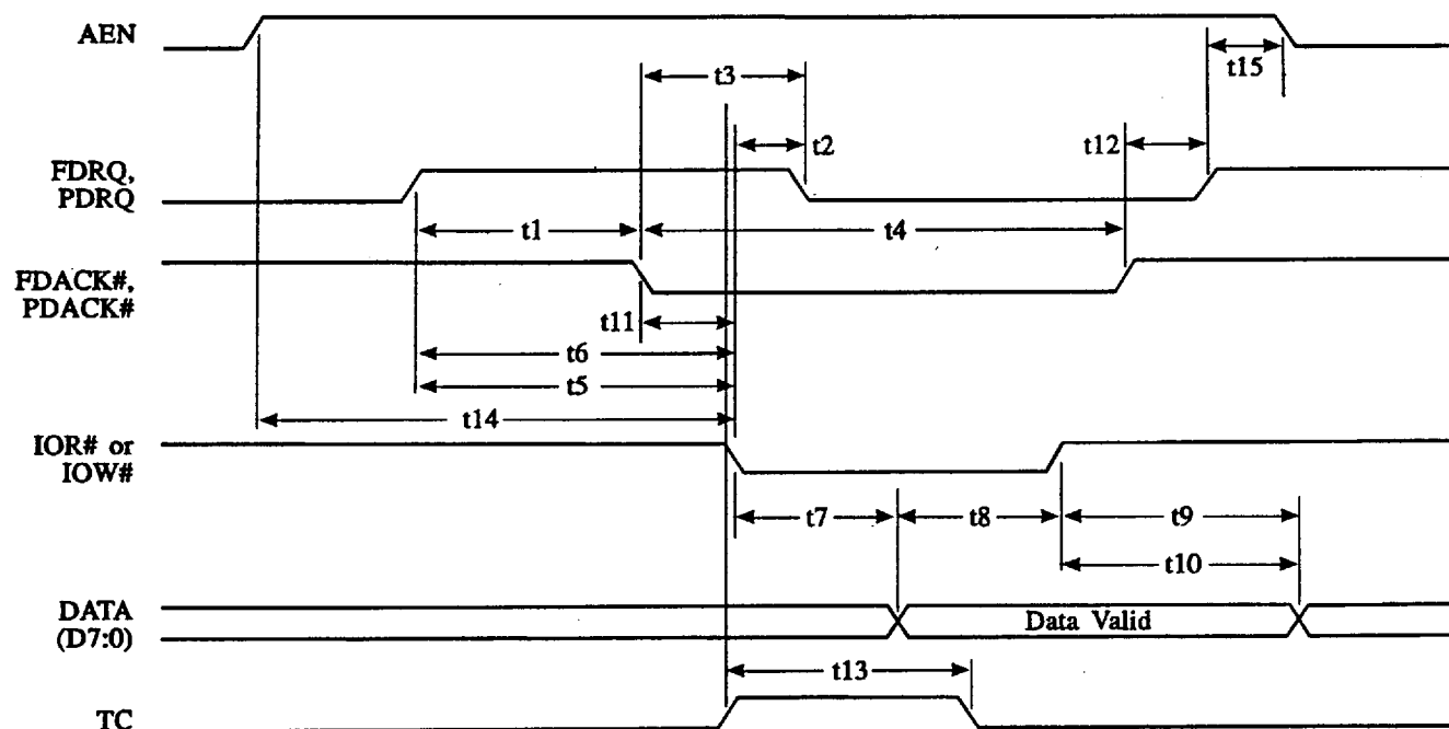
DMA Timing
