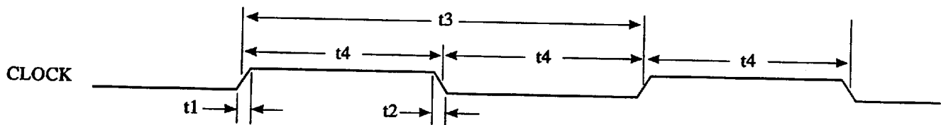
Clock Timing
