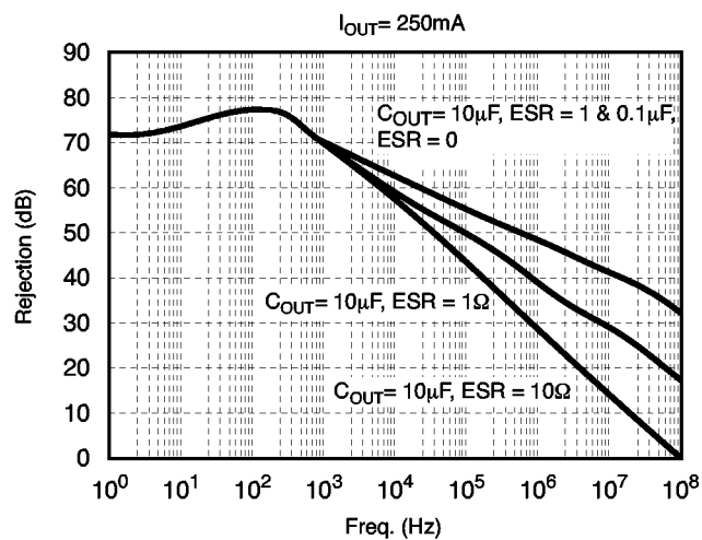
Ripple Rejection
