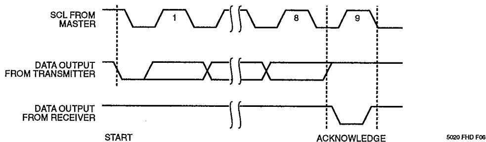
Figure 4. Acknowledge Timing
