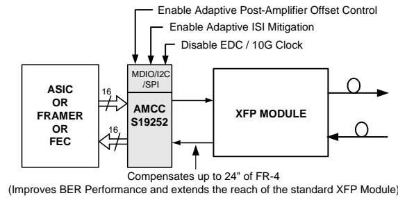
Figure 2. XFP Application Block Diagram
