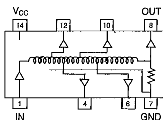
P Internal wiring
