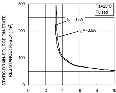
Fig.10 Static Drain-Source On-State Resistance vs. Gate-Source Voltage
