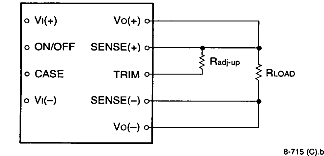
Figure 24. Circuit Configuration to Increase Output Voltage
