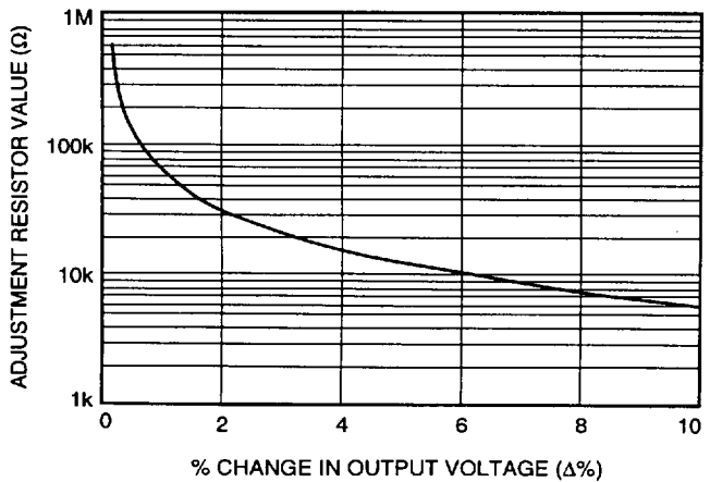
Figure 25. Resistor Selection for Increased Output Voltage
