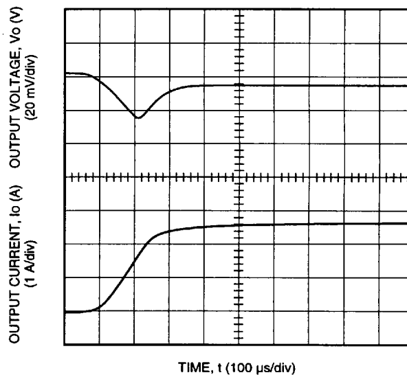
Figure 15. Typical JW150D Transient Response to Step Increase in Load at Room Temperature and 48 V Input (Waveform Averaged to Eliminate Ripple Component.)
