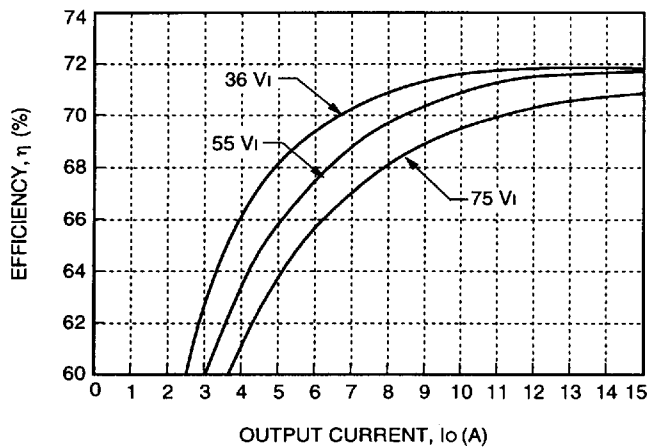
Figure 10. Typical JW075D Converter Efficiency vs. Output Current at Room Temperature
