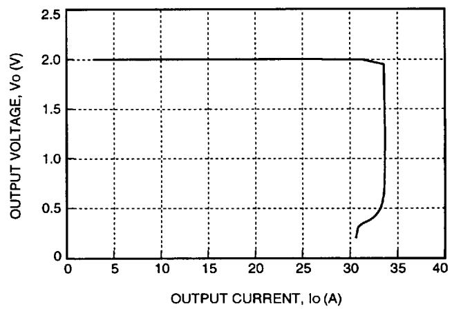
Figure 8. Typical JW150D Output Characteristics at Room Temperature, V_{IN} = 48 V
