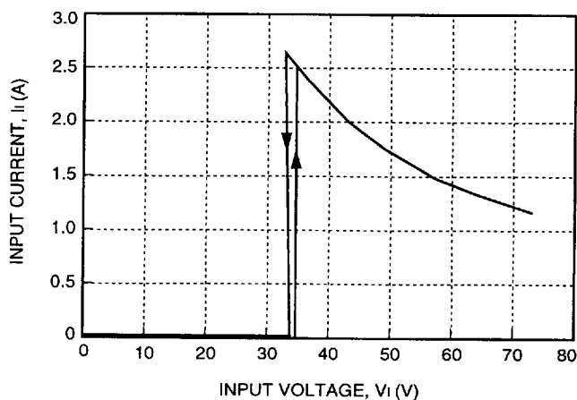
Figure 4. Typical JW150D Input Characteristics at Room Temperature, I_o = 30 A
