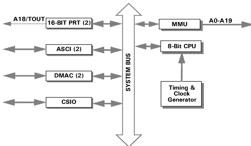
Z8S180 CORE PROCESSOR BLOCK DIAGRAM
