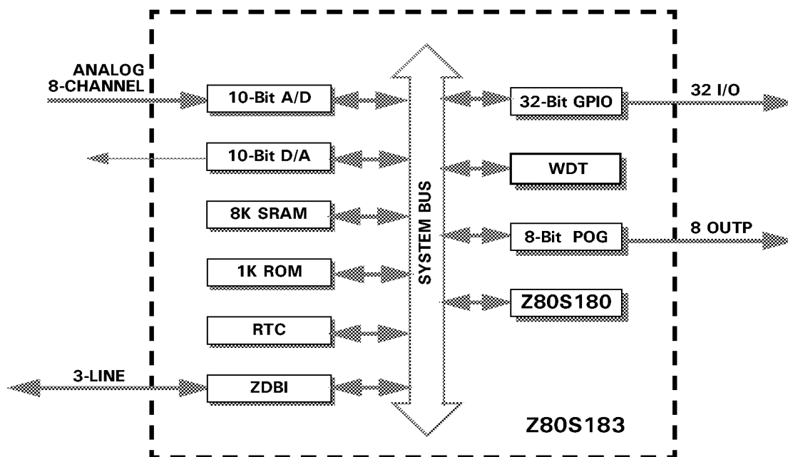
Z80S183 BLOCK DIAGRAM
