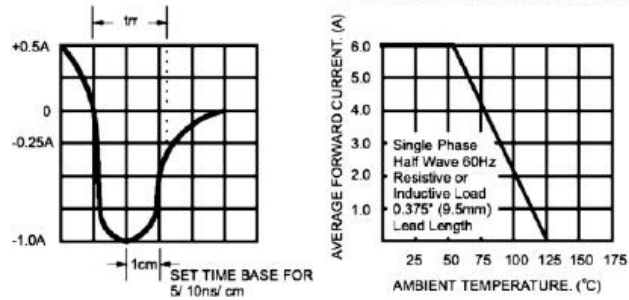
FIG.2- MAXIMUM AVERAGE FORWARD CURRENT DERATING
