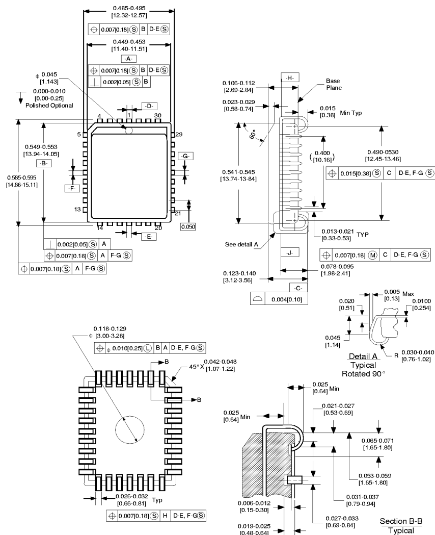
32-Lead PLCC Package Order Number NM27C020V Package Number VA32A
