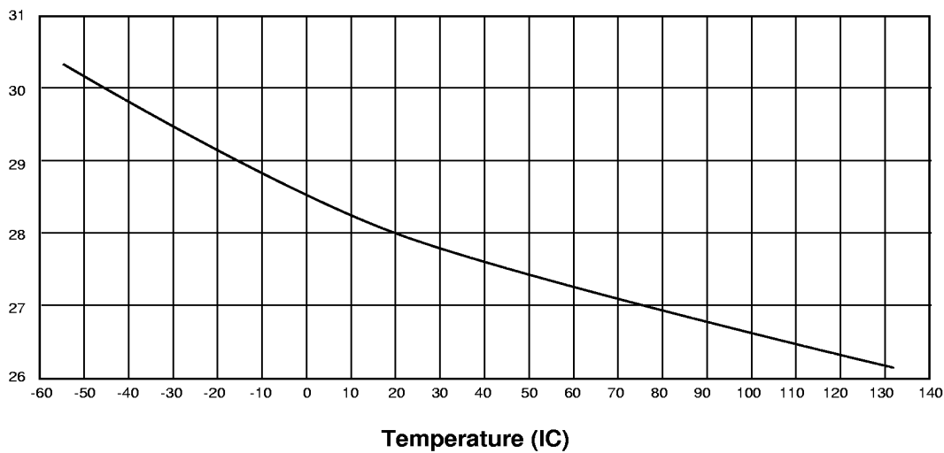
I_{CC} vs. Temperature
