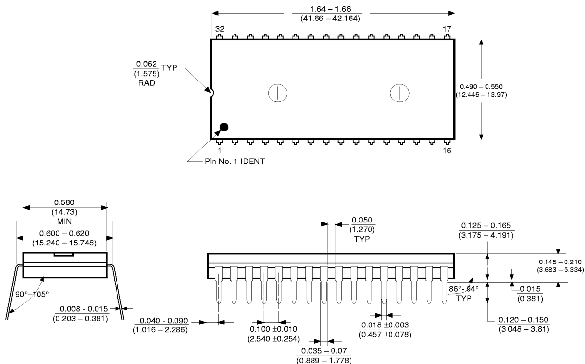
32-Lead PDIP Package Order Number NM27C020N
