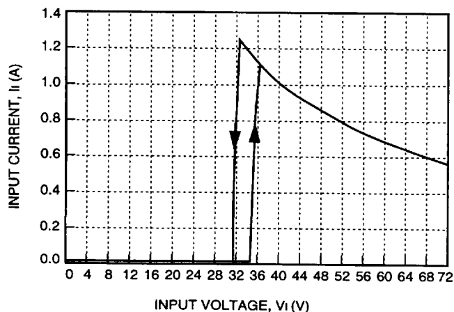
Figure 1. Typical JW050F Input Characteristics at Room Temperature, I_o = 10 A
