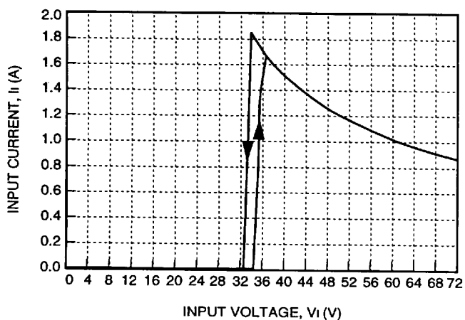
Figure 2. Typical JW075F Input Characteristics at Room Temperature, I_o = 15 A
