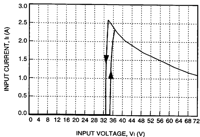
Figure 3. Typical JW100F Input Characteristics at Room Temperature, I_o = 20 A
