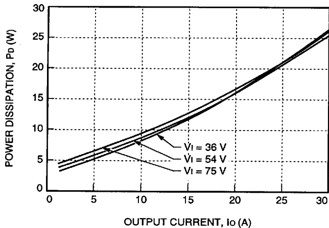
Figure 30. JW150F Power Dissipation vs. Output Current
