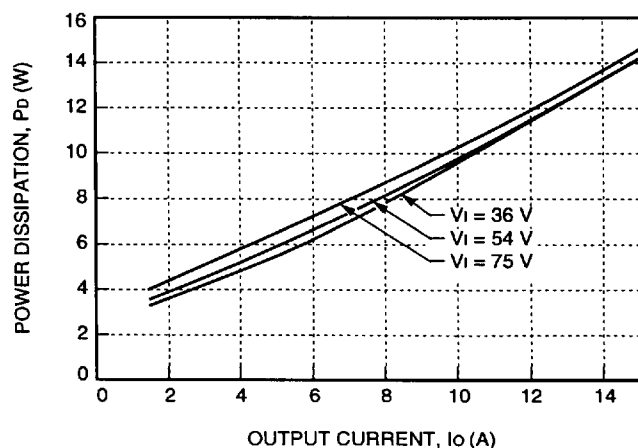
Figure 28. JW075F Power Dissipation vs. Output Current
