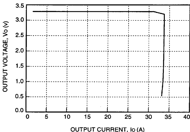
Figure 8. Typical JW150F Output Characteristics at Room Temperature, V_i = 48 V
