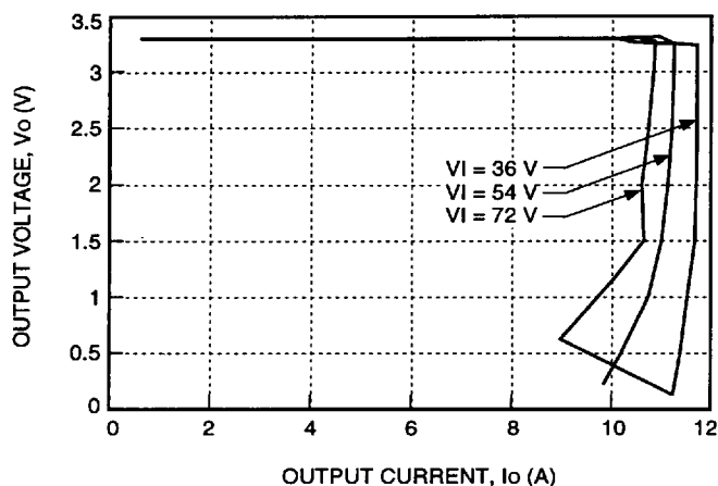
Figure 5. Typical JW050F Output Characteristics at Room Temperature, V_i = 48 V
