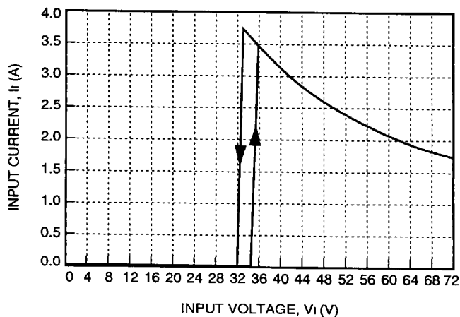
Figure 4. Typical JW150F Input Characteristics at Room Temperature, I_o = 30 A
