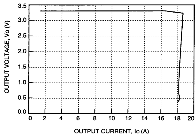
Figure 6. Typical JW075F Output Characteristics at Room Temperature, V_i = 48 V
