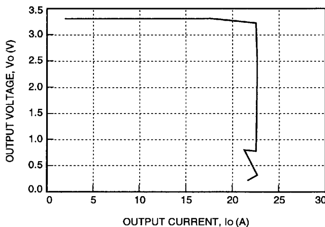
Figure 7. Typical JW100F Output Characteristics at Room Temperature, V_i = 48 V
