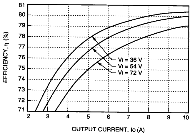
Figure 9. Typical JW050F Converter Efficiency vs. Output Current at Room Temperature
