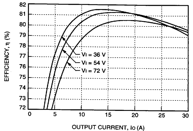
Figure 12. Typical JW150F Converter Efficiency vs. Output Current at Room Temperature
