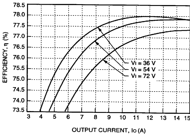
Figure 10. Typical JW075F Converter Efficiency vs. Output Current at Room Temperature
