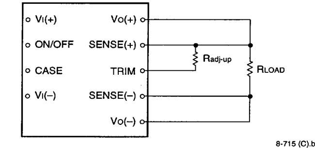
Figure 24. Circuit Configuration to Increase Output Voltage
