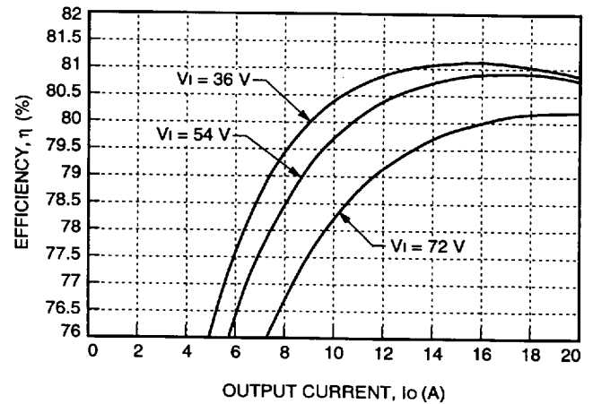
Figure 11. Typical JW100F Converter Efficiency vs. Output Current at Room Temperature
