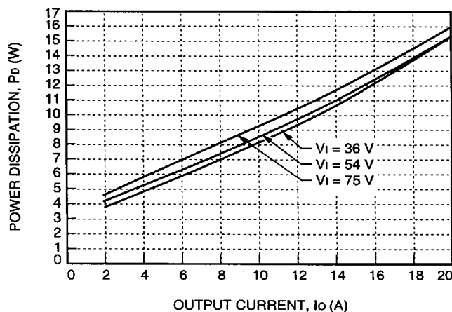
Figure 29. JW100F Power Dissipation vs. Output Current
