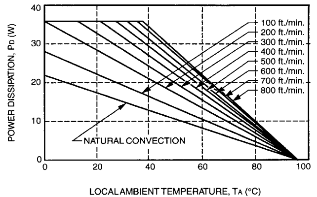
Figure 11. Power Derating vs. Local Ambient Temperature and Air Velocity
