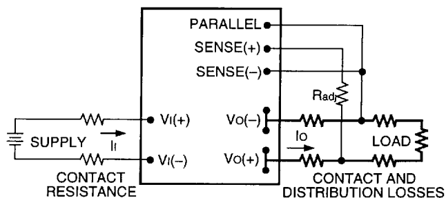
Figure 6. Circuit Configuration to Adjust Output Voltage.
