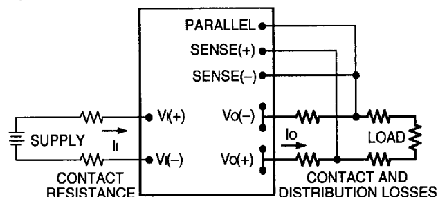
Figure 3. Effective Circuit Configuration for Single-Module Remote Sense Operation
