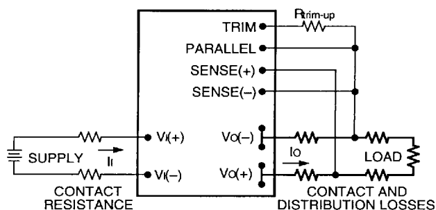
Figure 4. Circuit Configuration to Trim Up Output Voltage
