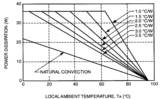
Figure 12. Power Derating vs. Local Ambient Temperature and Heat Sink Resistance
