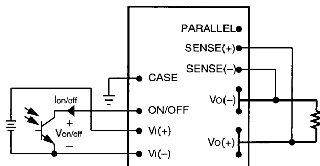
Figure 8. Remote On/Off Implementation
