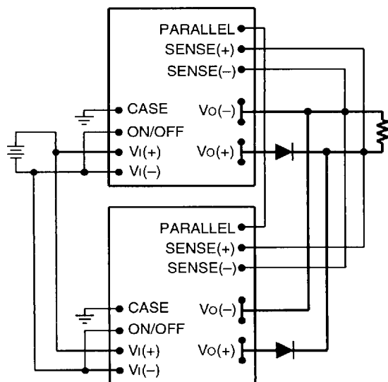
Figure 7. Wiring Configuration for Redundant Parallel Operation
