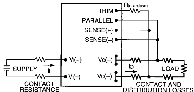
Figure 5. Circuit Configuration to Trim Down Output Voltage
