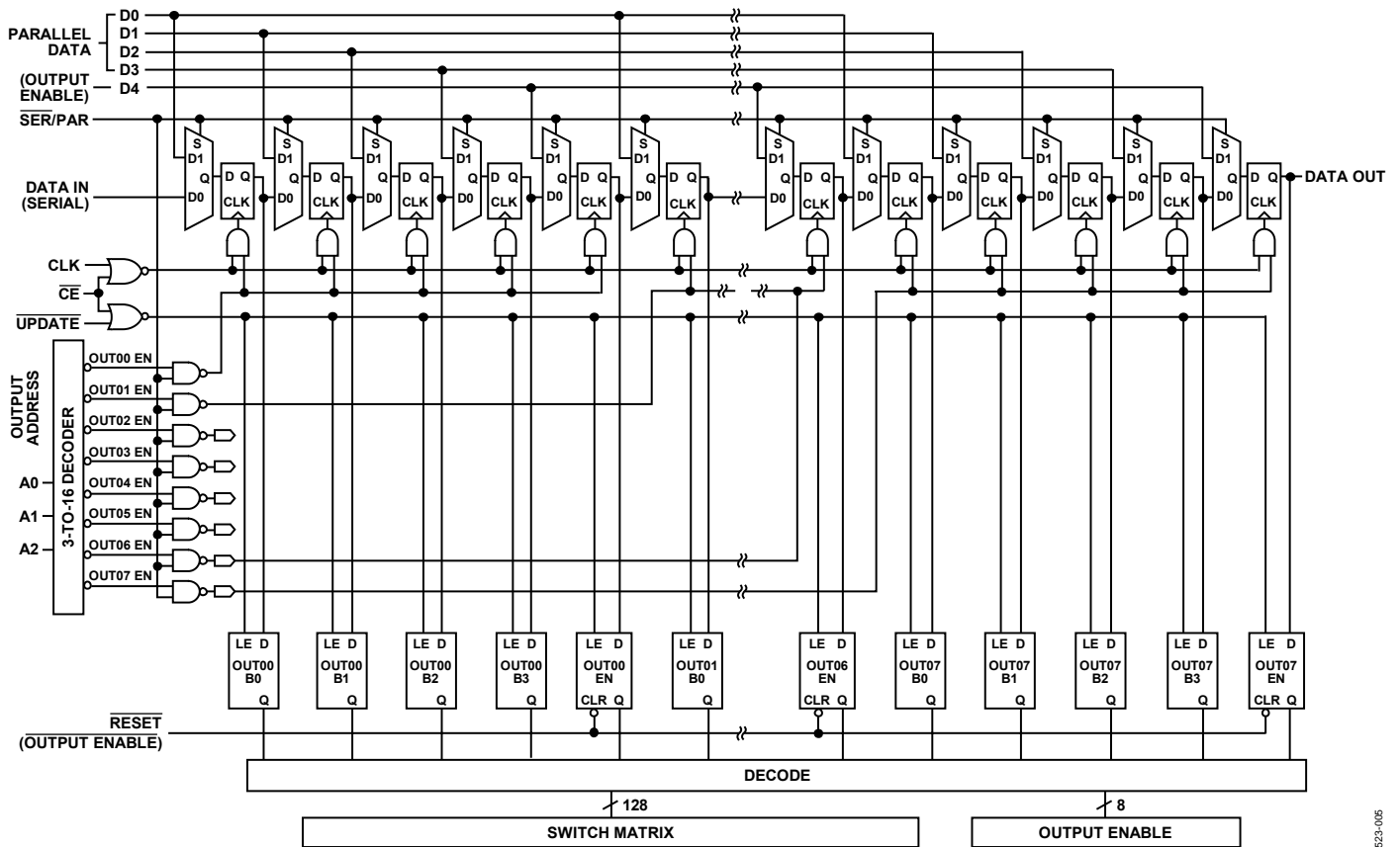
Figure 5. Logic Diagram
