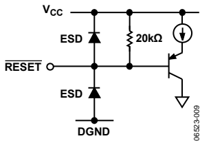
Figure 9. Reset Input
