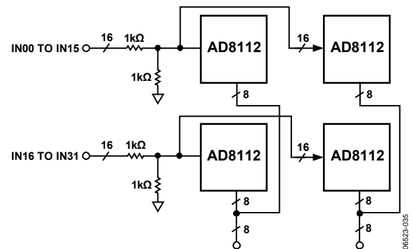
Figure 46. 32 \times 16 Audio Crosspoint Array Using Four AD8112s
