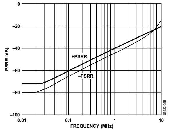
Figure 33. PSRR vs. Frequency, V_S = \pm 12 V
