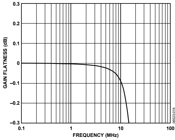
Figure 18. Large-Signal Gain Flatness, V_S = \pm 5 V , R_L = 150 \Omega , V_{OUT} = 2 V_{p-p}
