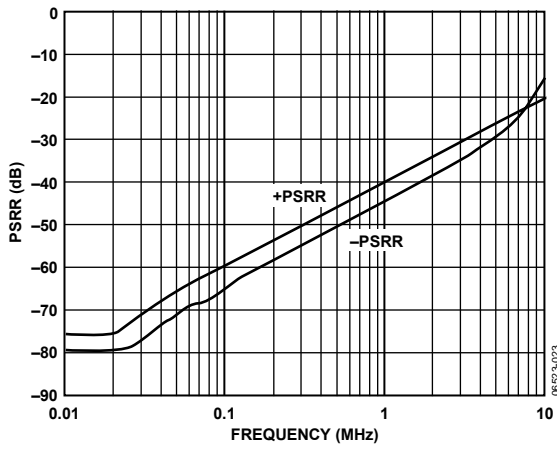
Figure 30. PSRR vs. Frequency, V_S = \pm 5 V
