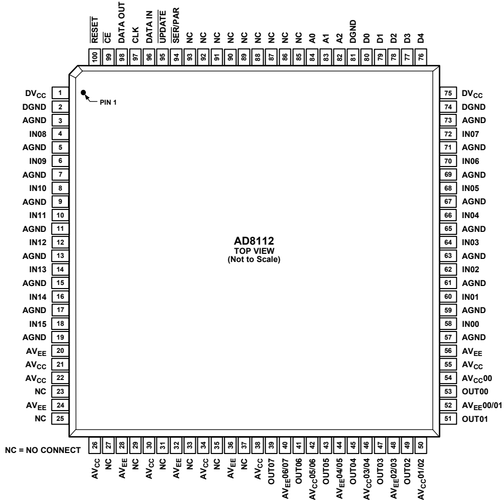
Figure 6. Pin Configuration
