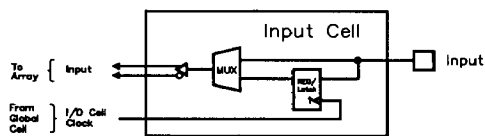
Figure 6. PA7040 Input Cell (INC)
