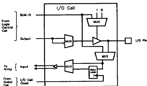
Figure 5. PA7040 I/O Cell (IOC)
