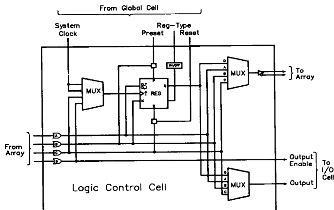
Figure 4. PA7040 Logic Control Cell (LCC)
