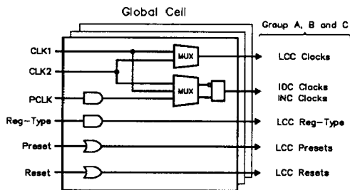
Figure 7. PA7040 Global Cell
