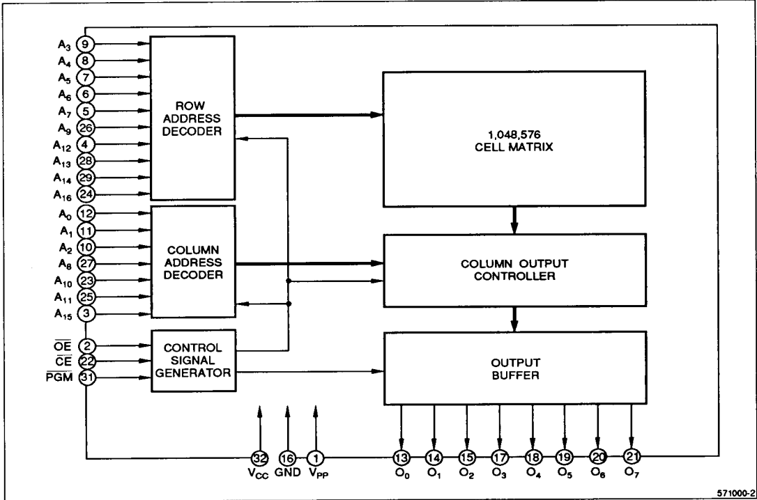
Figure 2. LH571000/J Block Diagram
