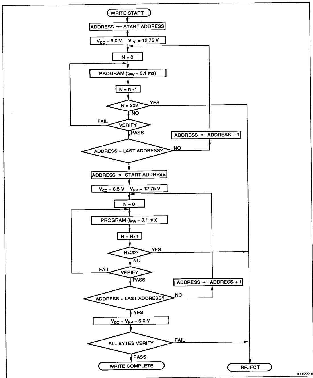
Figure 6. Programming Flowchart
