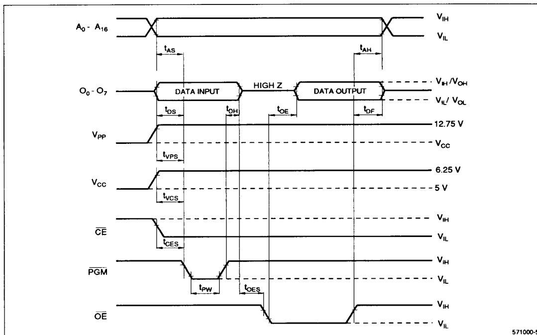
Figure 5. Timing Diagram (Program Mode)
