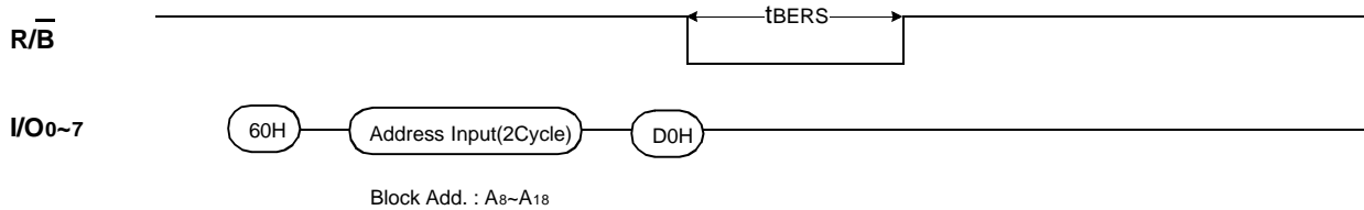
Figure 6. Block Erase Operation
