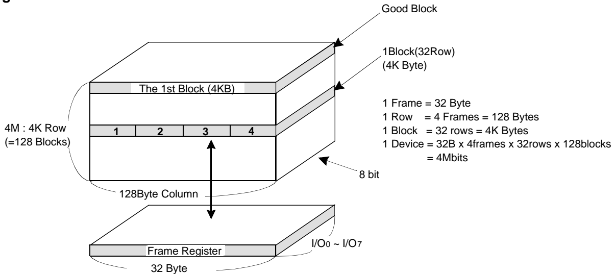
Figure 2. ARRAY ORGANIZATION
