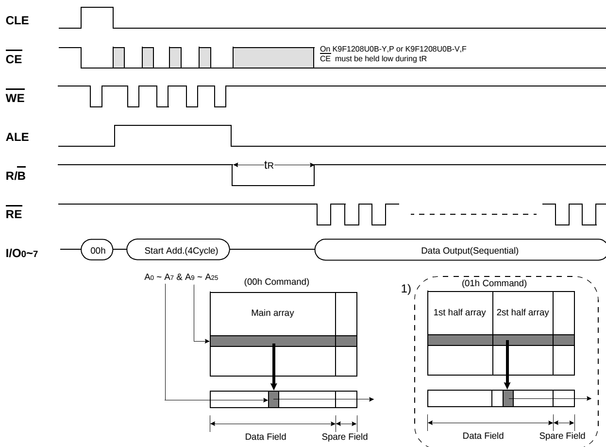
Figure 7. Read1 Operation
