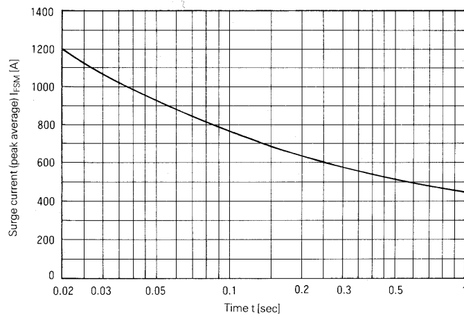
Surge Current
