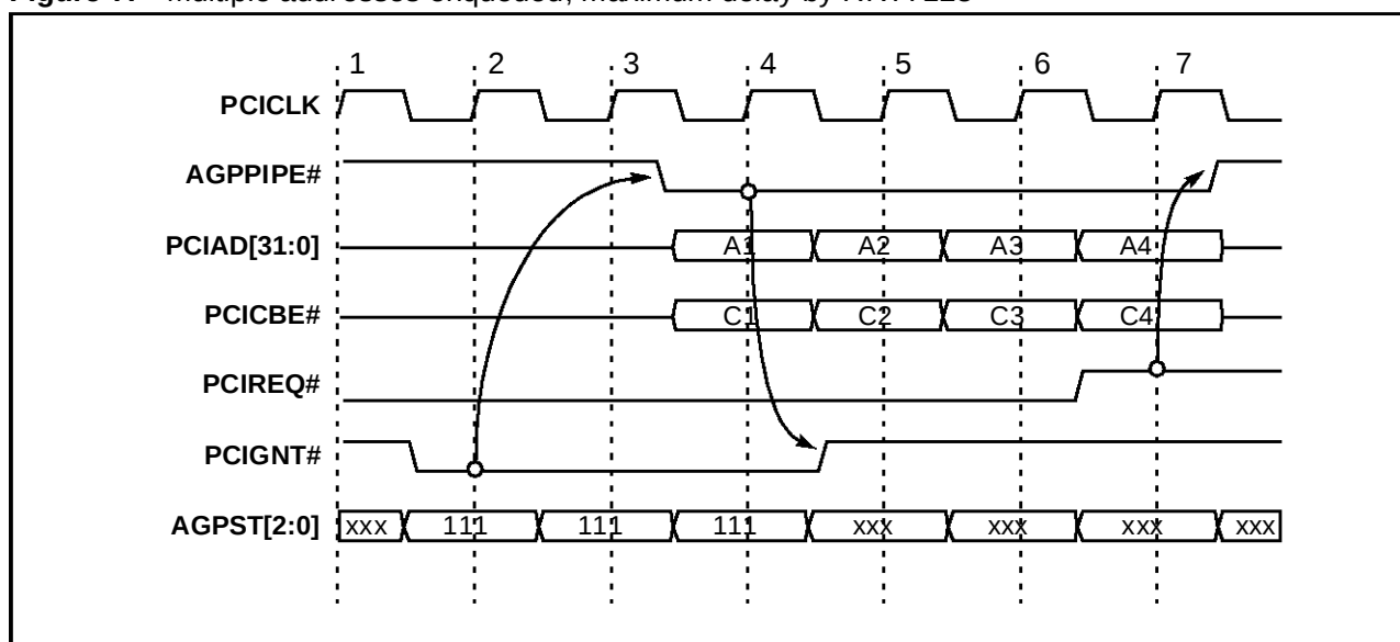
Figure 7. Multiple addresses enqueue, maximum delay by RIVA 128
