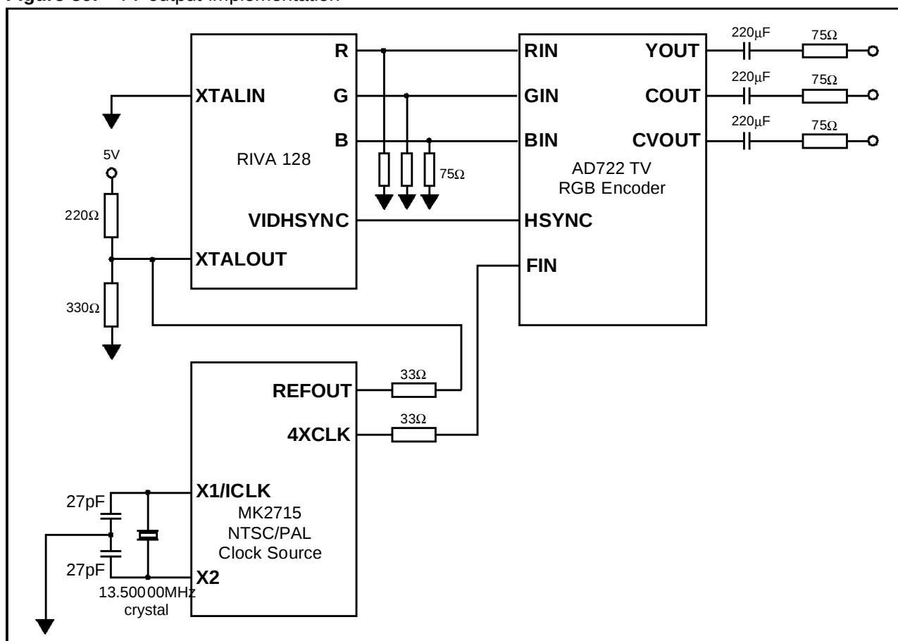
Figure 59. TV output implementation
