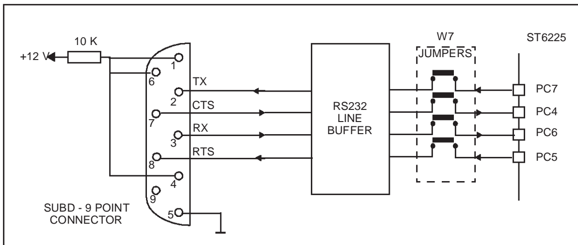
Figure 4: RS-232 connections and line allocations
