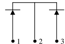
CC - COMMON CATHODE
