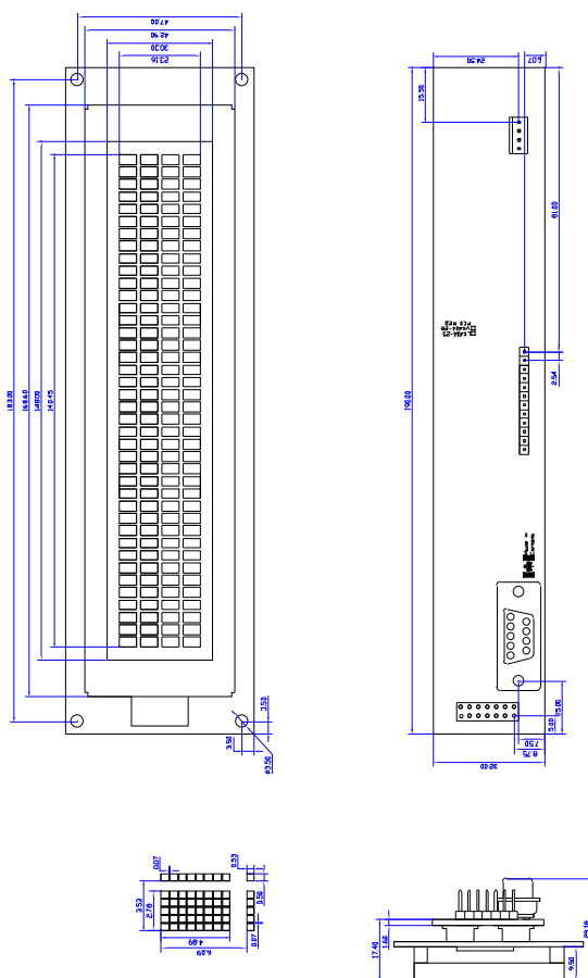
Figure 20: Physical Diagram
