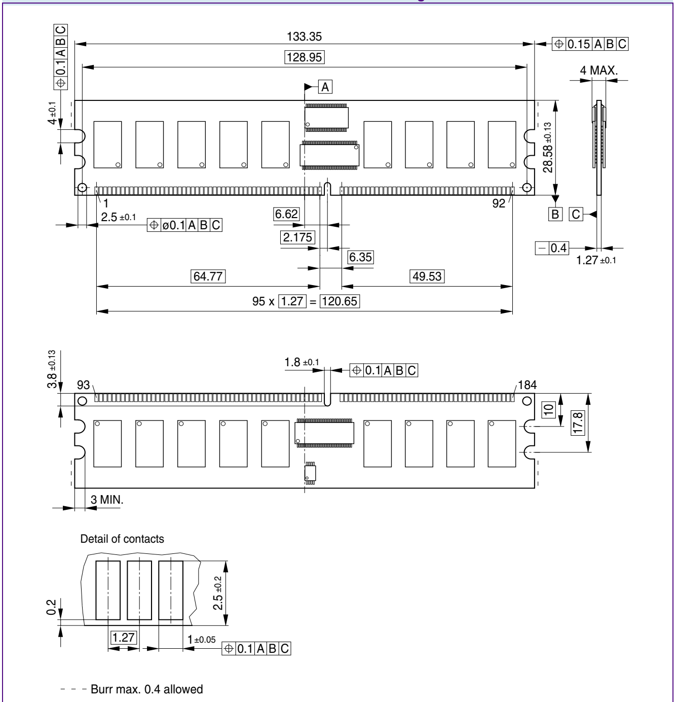
FIGURE 3 Package Outline Raw Card B - L-DIM-184-23-2
