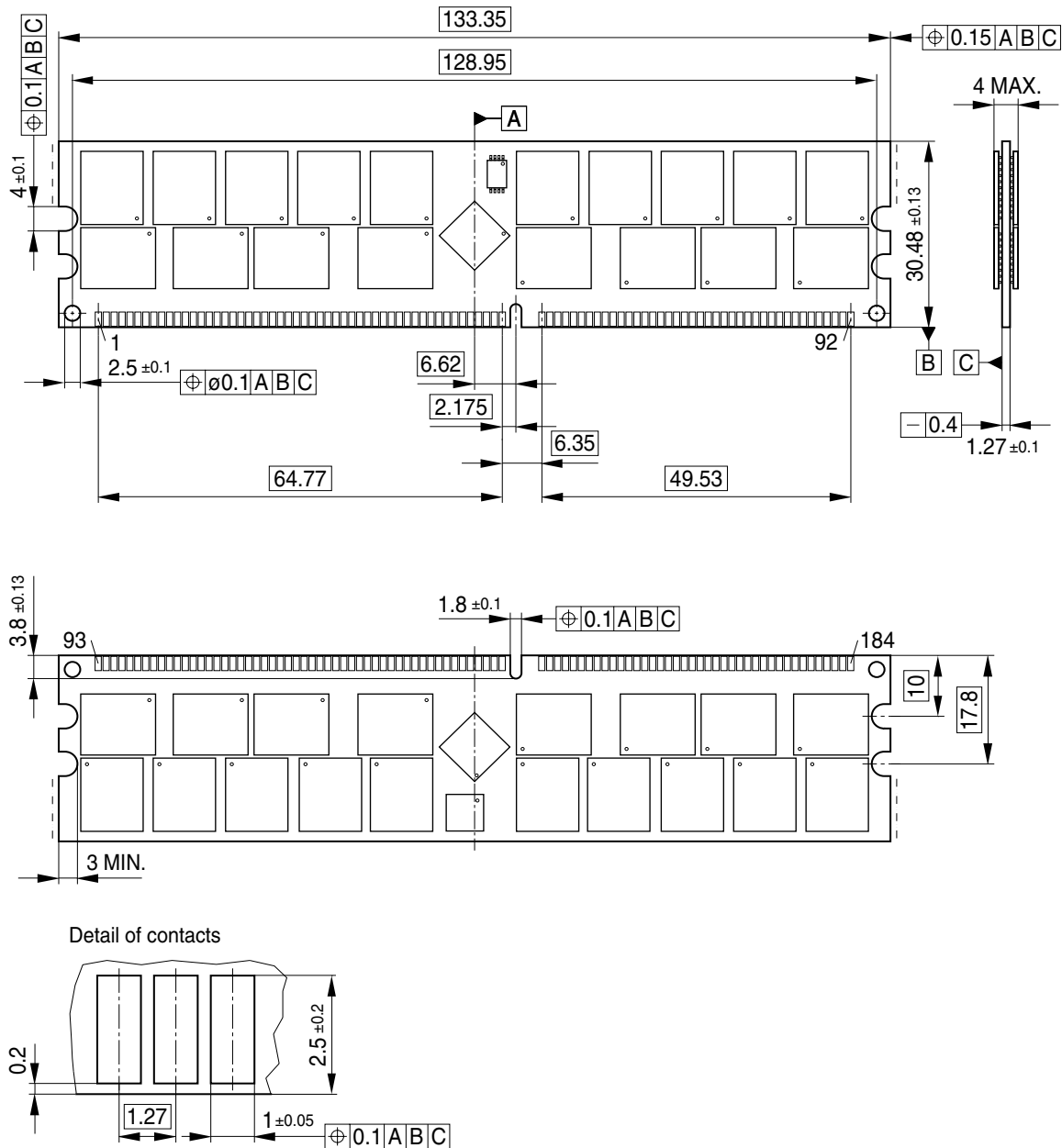
FIGURE 4 Package Outline Raw Card F – L-DIM-184-25
