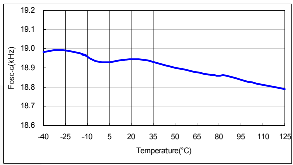
Figure 15. f_{OSC-G} vs. Temperature
