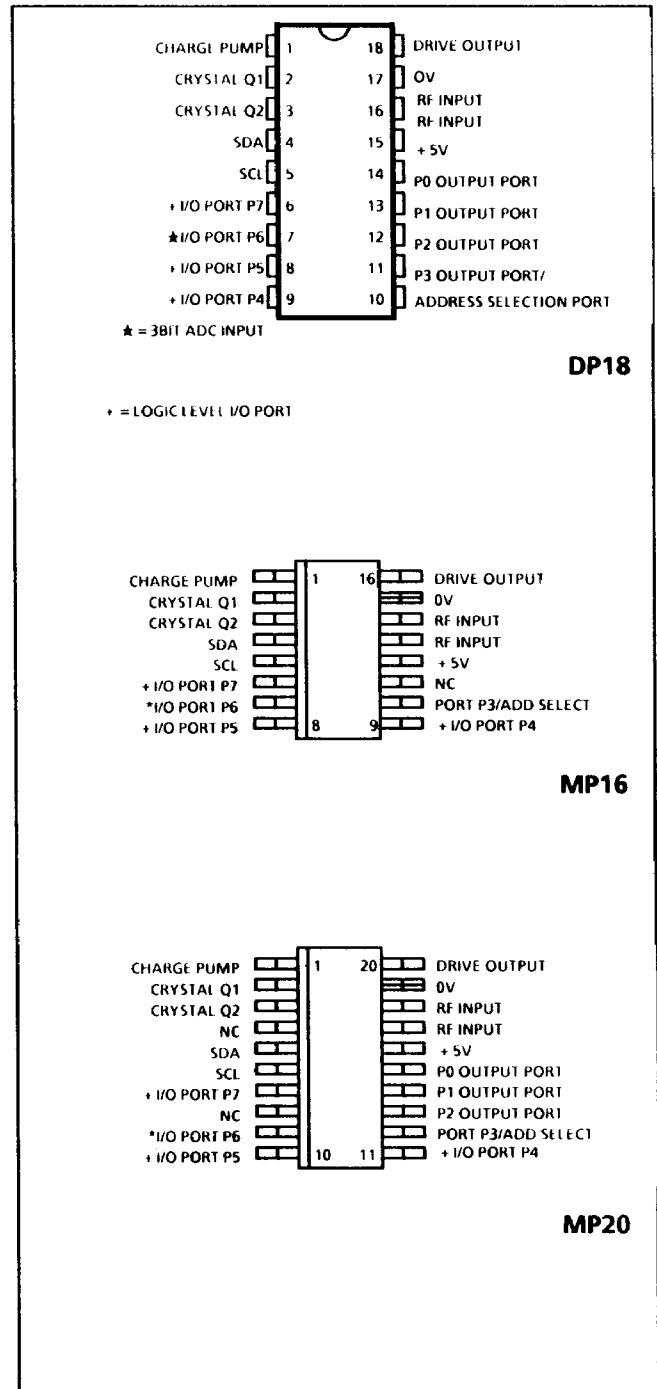
Fig.1 Pin Connections
