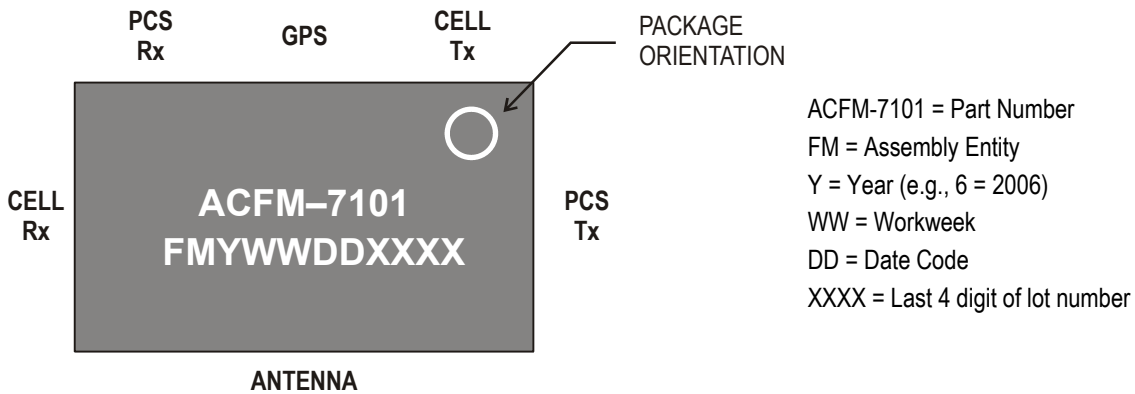
Figure 32. Package Marking.
