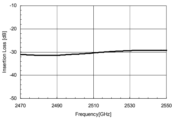
Figure 25. Cellular Tx-Rx Isolation at Tx Third Harmonic.
