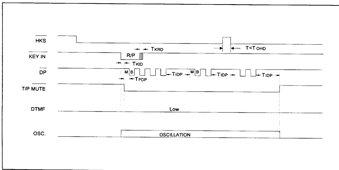
Figure 1(b) Pulse Mode Auto Dialing Timing Diagram
