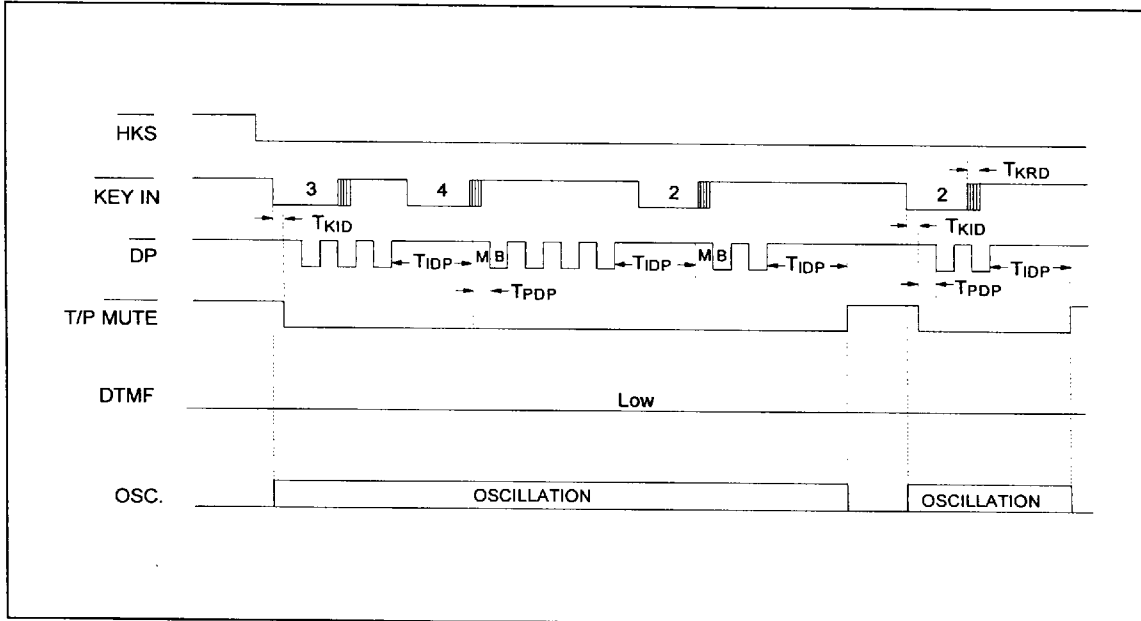
Figure 1(a) Normal Dialing Timing Diagram
