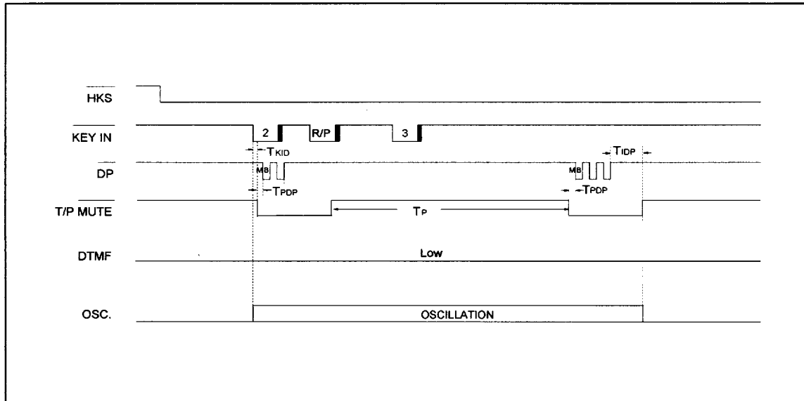
Timing Waveforms, continued
