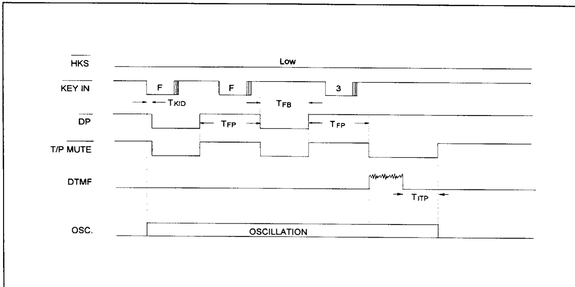
Figure 5. Flash Timing Diagram
