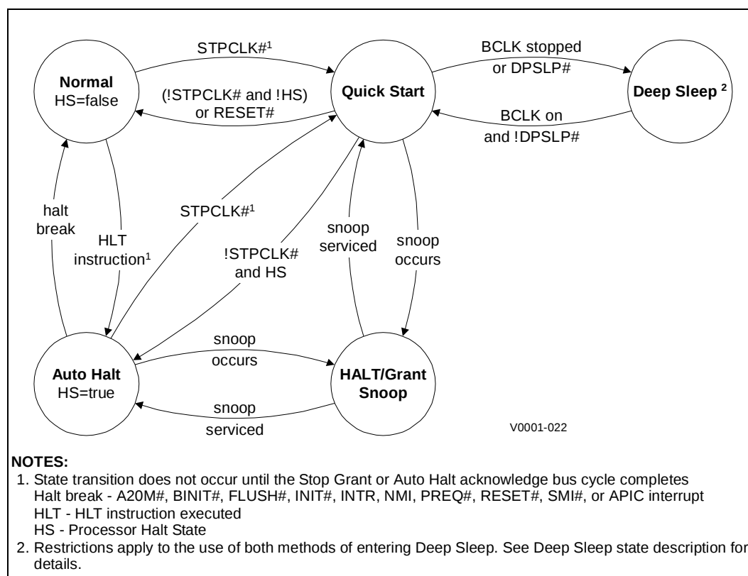
Figure 1. Clock Control States
