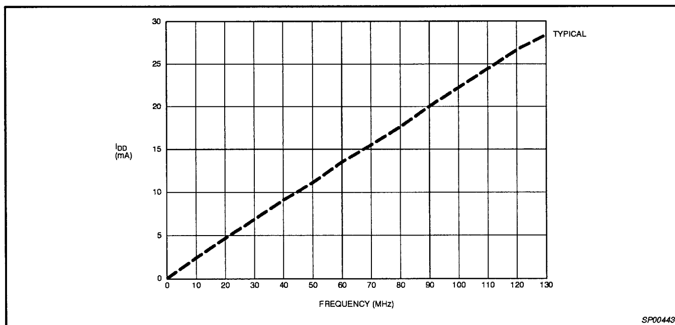
Figure 5. I_{DD} vs. Frequency @ V_{DD} = 3.3\text{V}
