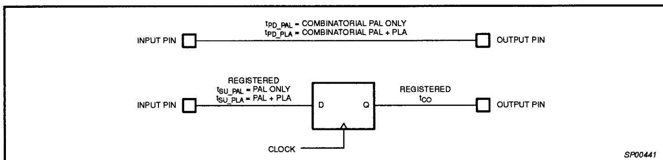
Figure 4. CoolRunner™ Timing Model
