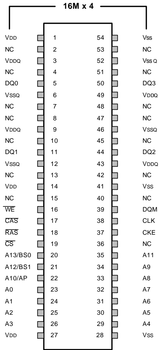
54-pin Plastic TSOP-II 400 mil
