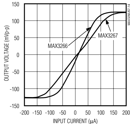
DC TRANSFER FUNCTION
