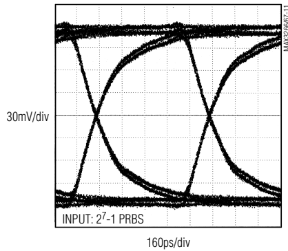
EYE DIAGRAM (INPUT = 1mA p-p )
