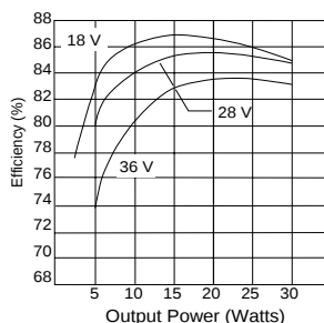
HR301-2812 Efficiency
