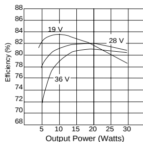
HR301-2805 Efficiency
