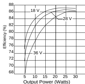
HR302-2815 Efficiency
