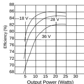
HR302-2812 Efficiency
