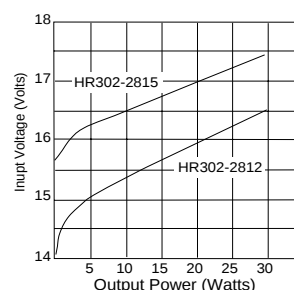
HR302-2812 and HR302-2815 Low Line Dropout
