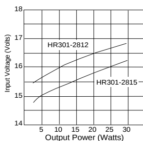
HR301-2812 and HR301-2815 Low Line Dropout
