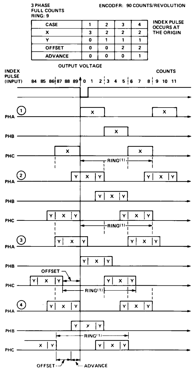
Figure 10. Commutator Configuration.
