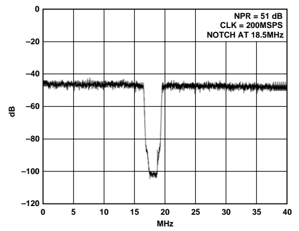
Figure 36. Noise Power Ratio Plot (200 MSPS Grade)
