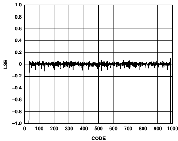
Figure 32. Typical DNL Plot (AIN = 10.3 MHz @ -0.5 dBFS) 170/200 MSPS
