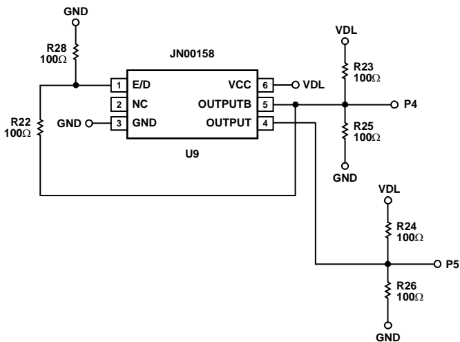
Figure 46. Evaluation Board Schematic (continued)
