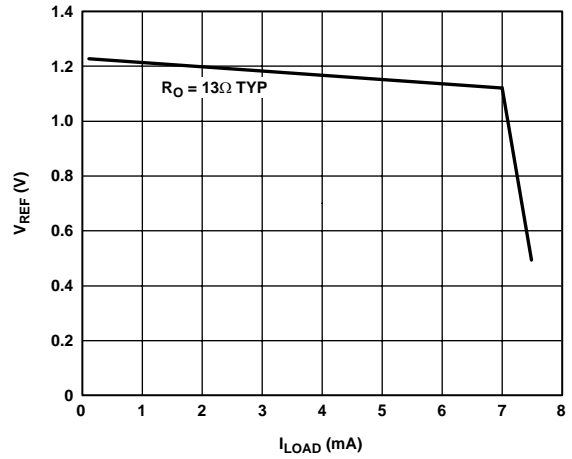
Figure 25. VREF vs. ILOAD (Both Speed Grades)
