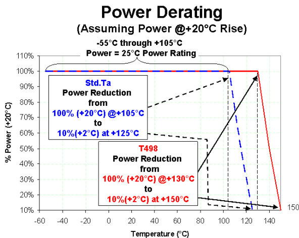
Figure 6. Power derating to maximum temperatures.
