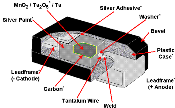
Figure 1. Structure of new T498 tantalum capacitor.
