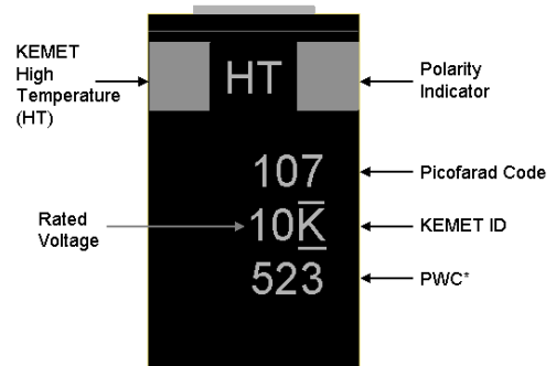
Figure 3. Component marking diagram for T498 capacitor.
