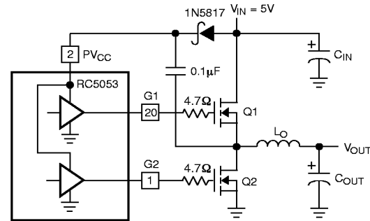
Figure 7. Doubling Charge Pump
