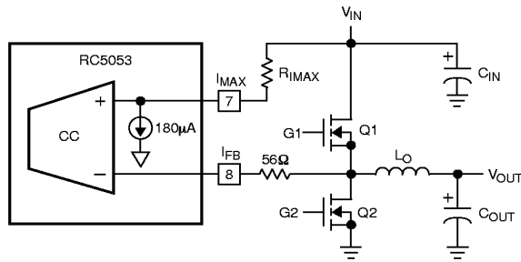
Figure 5. Current Limit Setting
