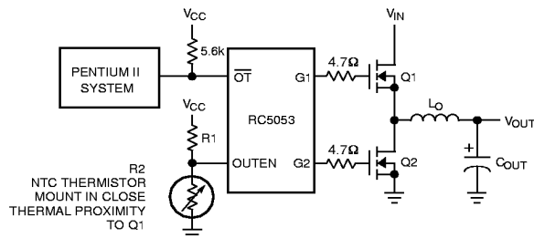
Figure 6. OUTEN Pin as a Thermistor Input
