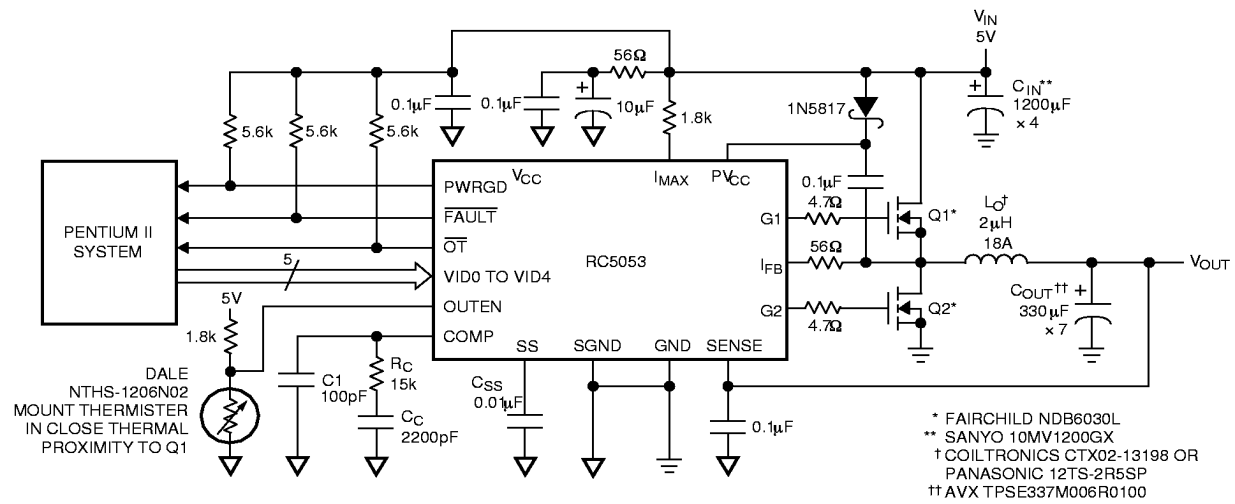
Figure 11. Single Supply RC5053 5V to 1.8V-3.5V Application with Thermal Monitor
