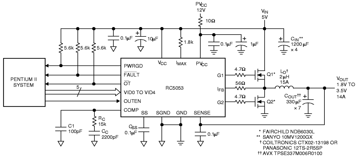
Figure 1. 5V to 1.8V-3.5V Supply Application
