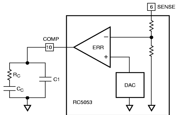
Figure 8. Compensation Pin Hook-Up
