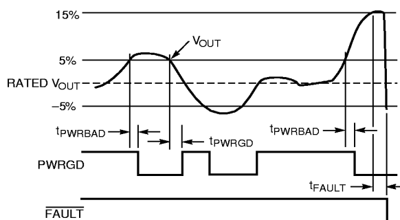
Figure 9. PWRGD and FAULT
