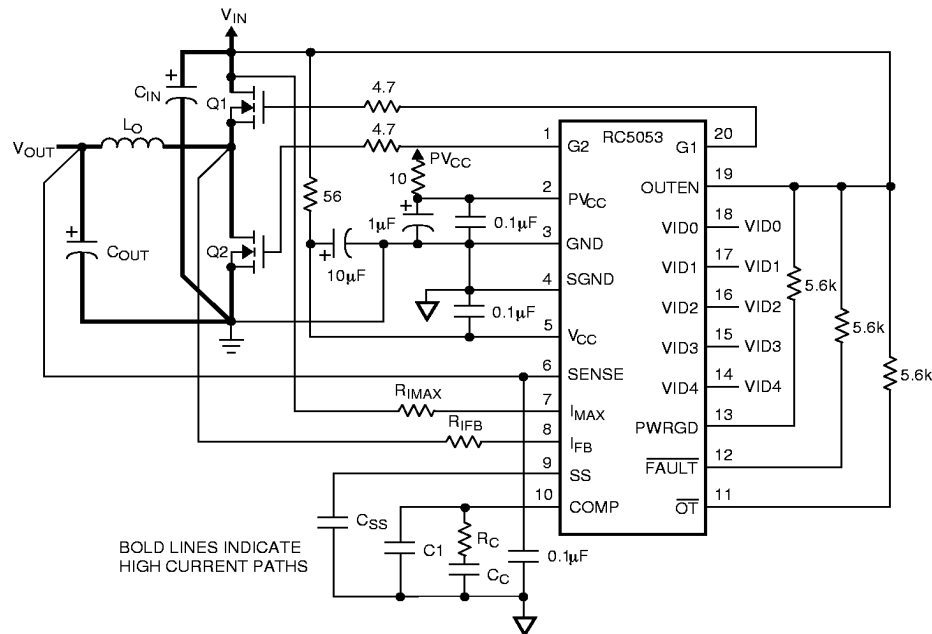
Figure 10. RC5053 Layout Diagram
