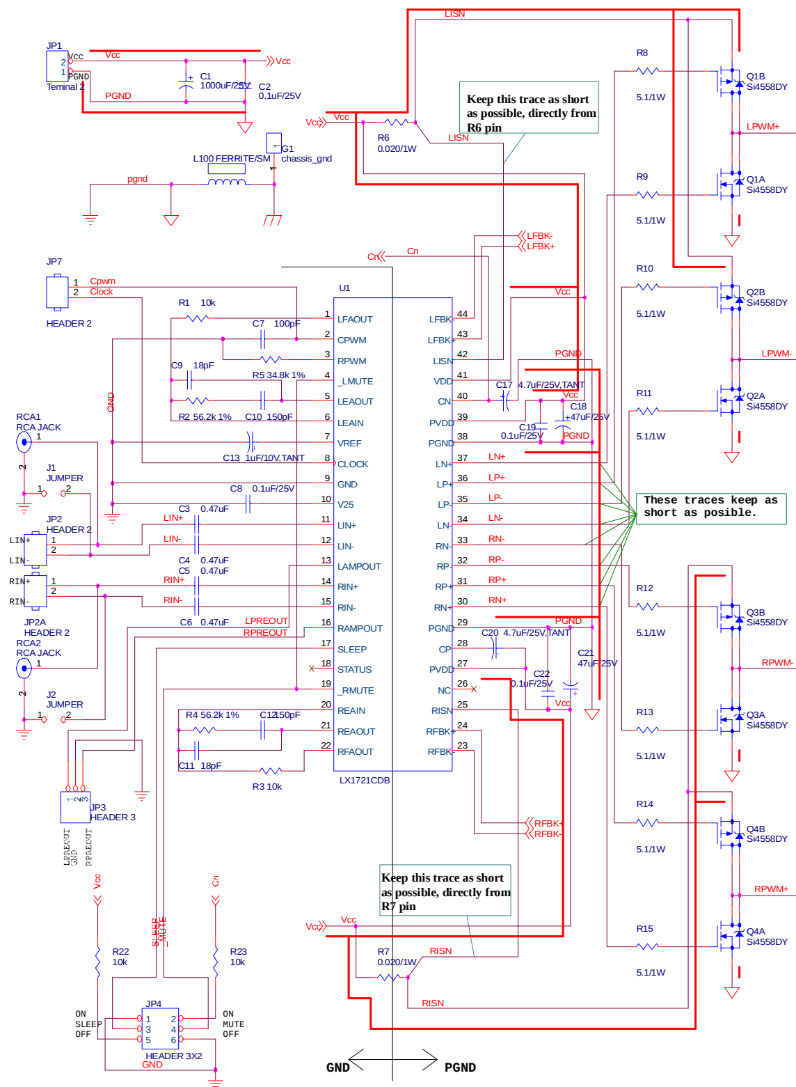
FIGURE 1A - LXE1721 SCHEMATIC (VIEW OF LX1721 SECTION)
