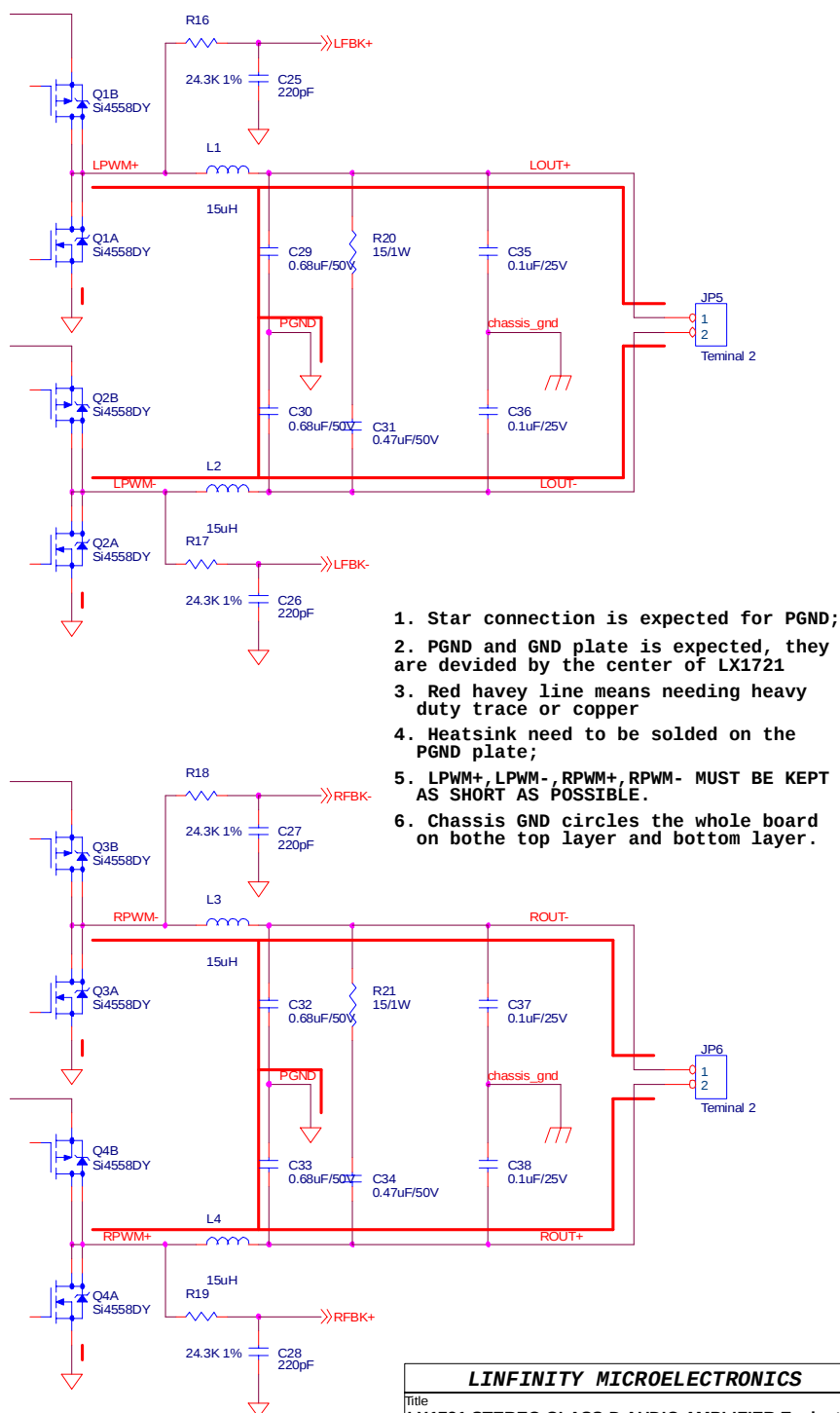
FIGURE 1B - LX1721 SCHEMATIC (VIEW OF OUTPUT SECTION)
