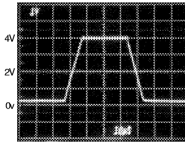
LARGE-SIGNAL TRANSIENT RESPONSE ( V_S = 5V, 0V )
