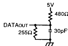
Figure 1. Output Load
