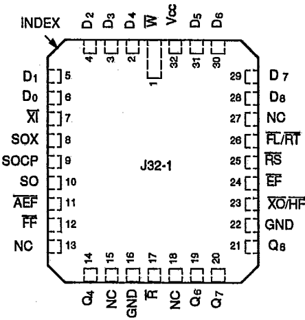
PLCC TOP VIEW
