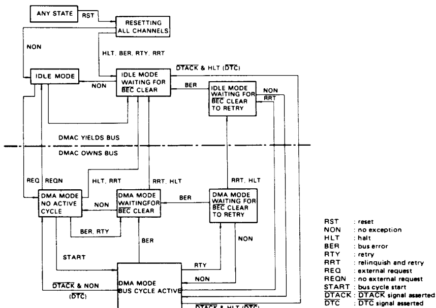
Figure 43 Bus Exception Flow Diagram
