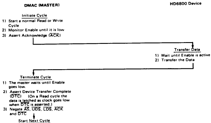
Figure 25 HD6800 Cycle Flowchart
