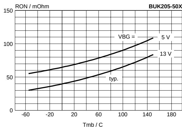
Fig.9. Typical on-state resistance, t_p = 300 \mu s . R_{ON} = f(T) ; parameter V_{BG} ; condition I_L = 1.5 A
