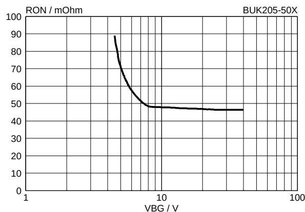
Fig.8. Typical on-state resistance, T_j = 25^\circ\text{C} . R_{ON} = f(V_{BG}) ; conditions: I_l = 7.5\text{ A} ; t_n = 300\text{ }\mu\text{s}
