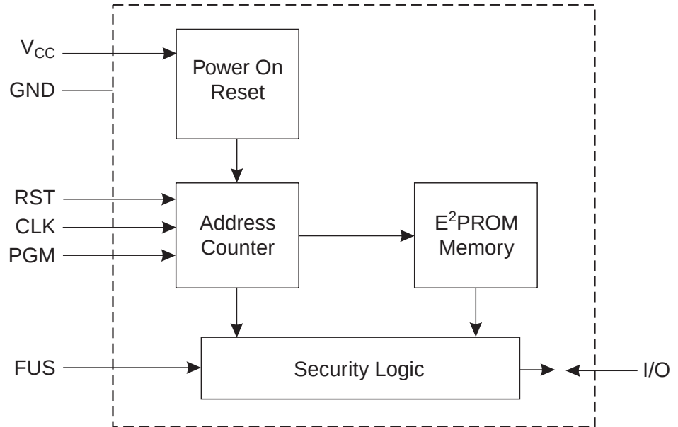
Figure 2. Block Diagram
