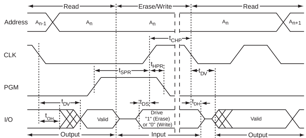
Figure 6. Erase/Write
