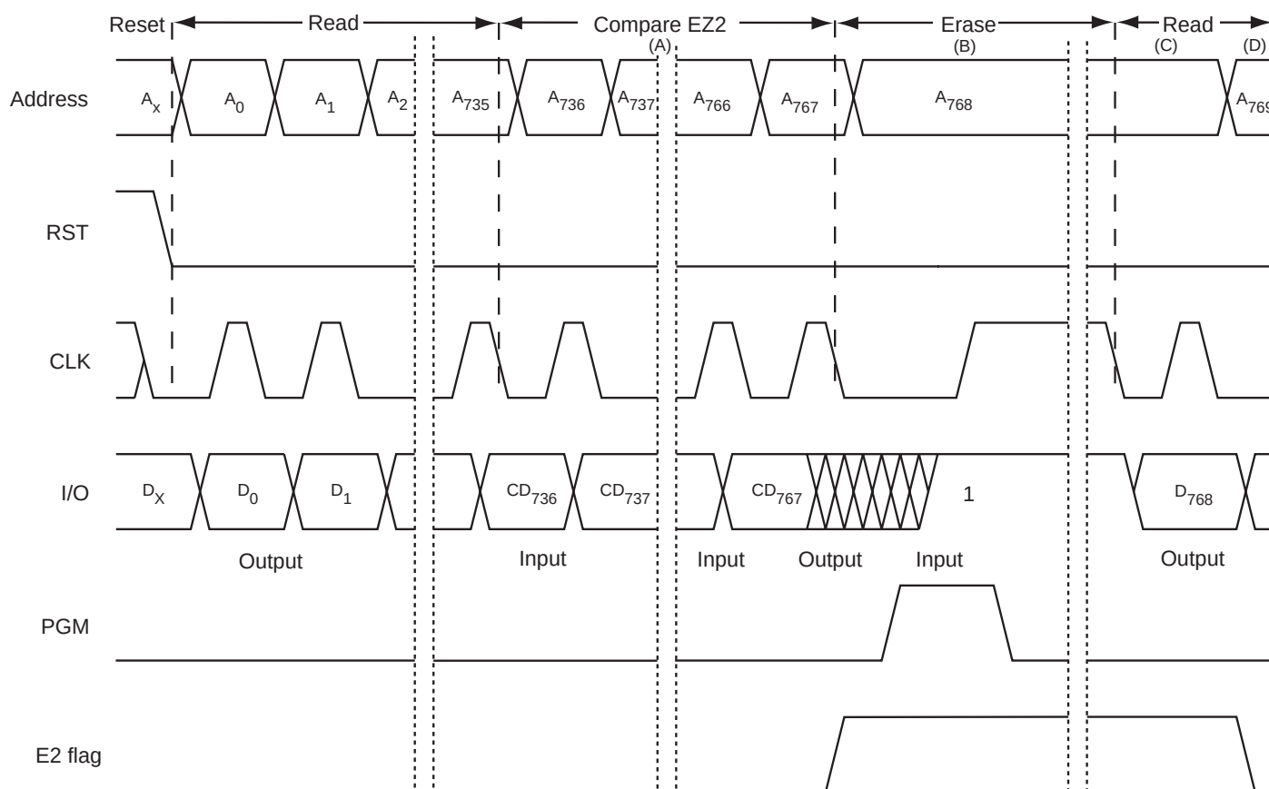
Figure 11. Erase Operation Application Zone 2 (AZ2) EC2 Function Disabled
