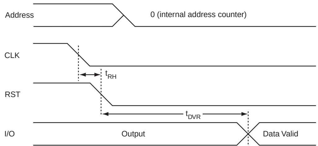
Figure 4. Reset
