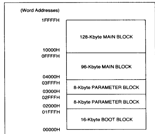
Figure 4. A28F200BX-B Memory Map
