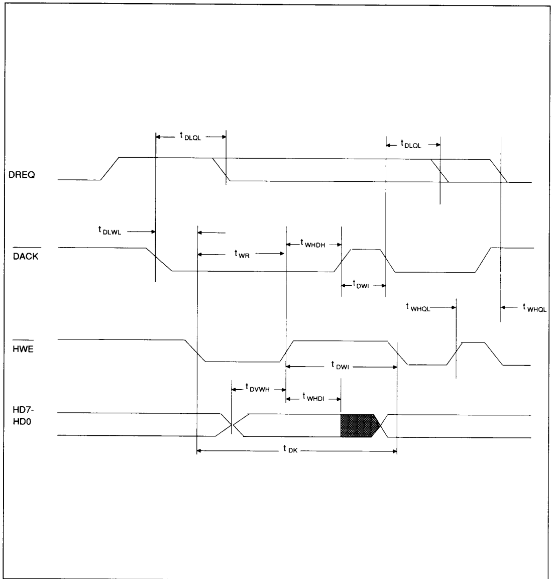
FIGURE 10. AT/XT HOST DMA WRITE TIMING
