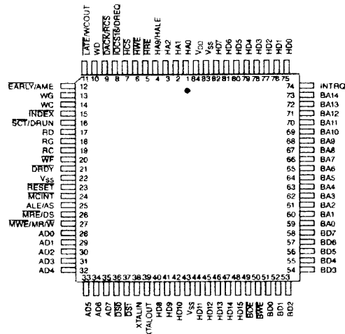
FIGURE 1. 84-PIN PLCC OR PQFP
