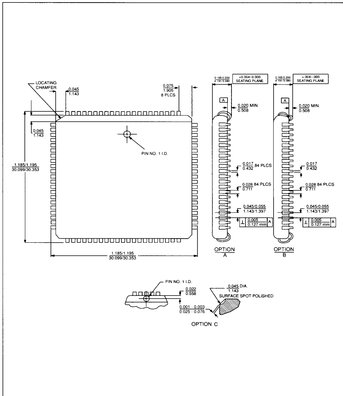
FIGURE 35. 84-PIN PLCC PACKAGE DIMENSIONS
