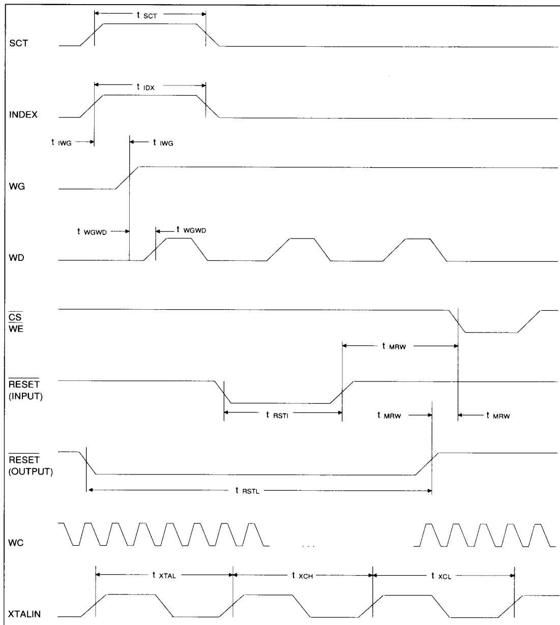
FIGURE 28. MISCELLANEOUS TIMING
