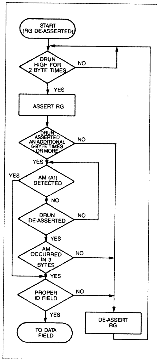
FIGURE 4. PLL CONTROL (ID FIELD)
