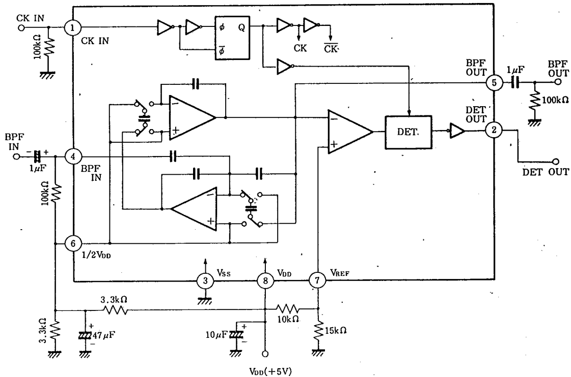
■ 応用回路例 / Application Circuit
