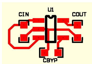
Figure 5. Fixed Mode
