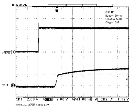
Shutdown Pin Delay
