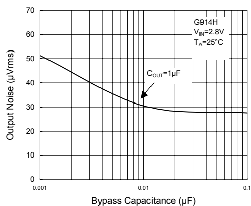
Output Noise vs. Bypass Capacitance
