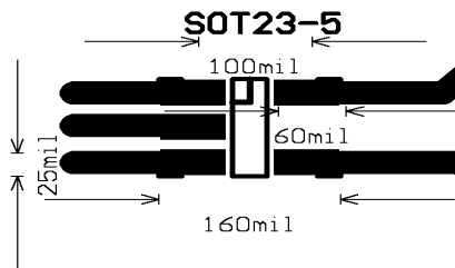
Figure 2. Recommended Minimum Footprint
