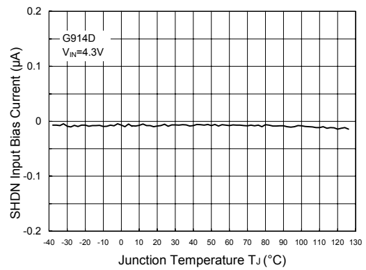
\overline{SHDN} Input Bias Current vs. Temperature
