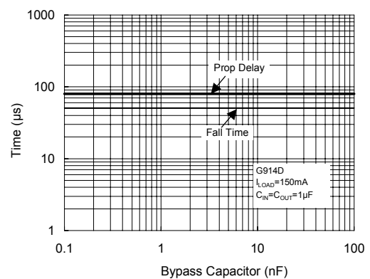
Turn-Off Time vs. Bypass Capacitance
