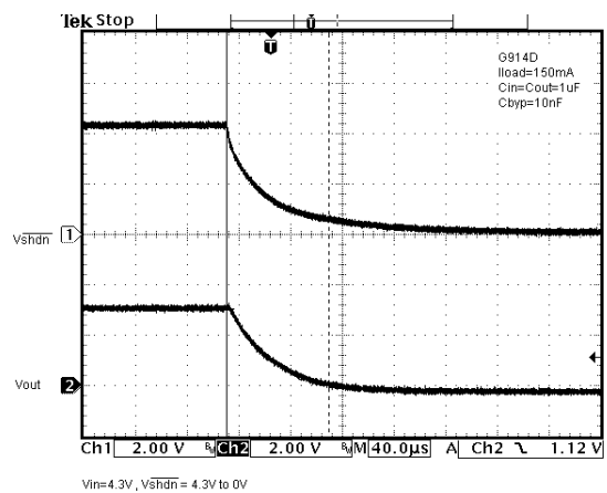
Shutdown Response Time
