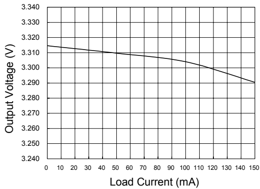
Output Voltage vs. Load Current
