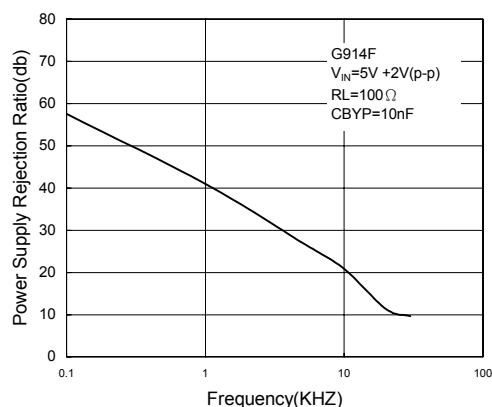
Power Supply Rejection Ripple
