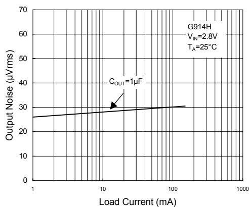
Output Noise vs. Load Current
