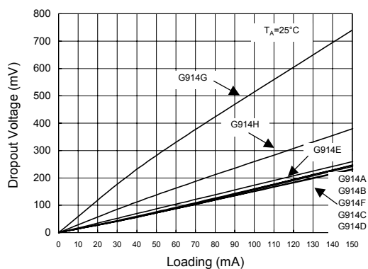
Dropout Voltage vs. Loading by G914X
