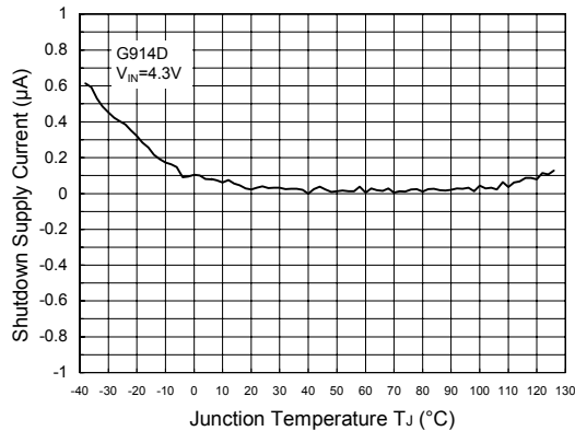
Shutdown Supply Current vs. Temperature
